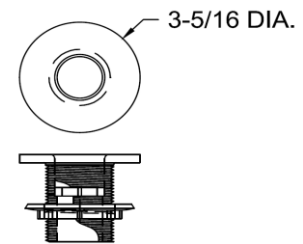
PSO3R SINK OUTLET WITH INTEGRAL TAILPIECE 1 1/2" N.P.T.
