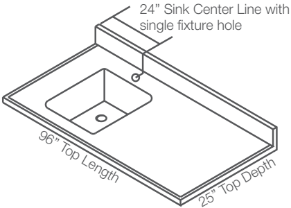
Sample Top with Dimensions - Top Style F
