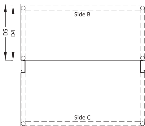
Example of Envision 4.0, 6" Upright Double Sided Workstation with (1) Bolt-on and (1) Frame/Table
