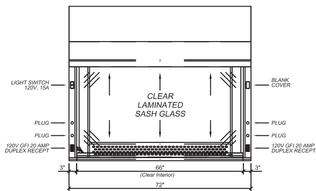
F-EXP II-72SIN - 72" Wide
