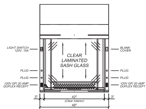
F-EXP II-48SIN - 48" Wide
