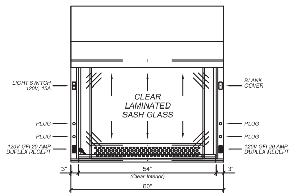
F-EXP II-60SIN - 60" Wide
