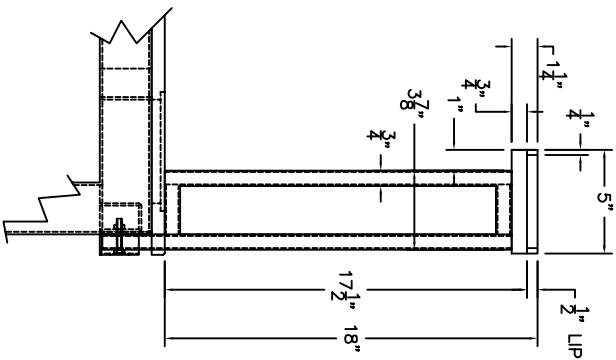
SHELF END VIEW
