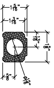
STANDARD FLEX-A-SCOPE MANIFOLD SECTION 6063-T5 ALUMINUM
